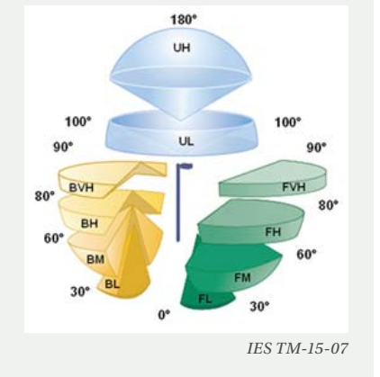
FIGURE 7. BUG System lighting zone specifications
