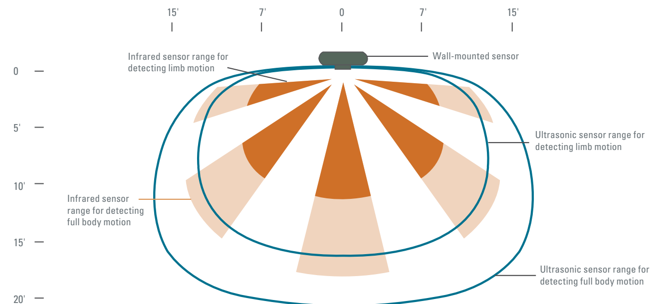
FIGURE 10. Various occupancy sensor configurations and ranges
