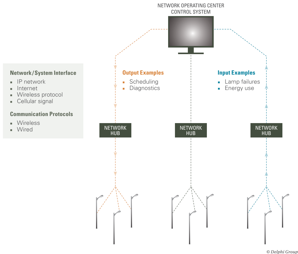
FIGURE 12. Network-controlled system
